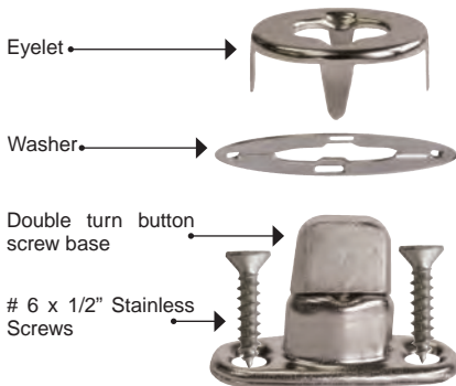
Osborne No. K4110 Turn Buttons
